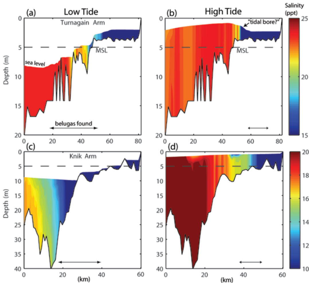
Figure 4. Cross section of salinity (color scale in ppt) during low (left panels) and high (right panels) tides for the Turnagain (upper panels) and Knik (lower panel) Arms, as simulated by the numerical model. The sections are along the deepest part of each arm. Mean sea level (MSL) is indicated by the dashed line. The ranges where belugas were observed in this study are indicated at the bottom of each panel.
